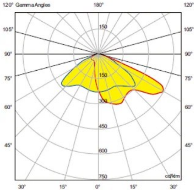
Tennis Court Type III (Standard)
