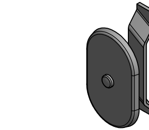
3.00 X 5.00 HAND HOLE COVER
