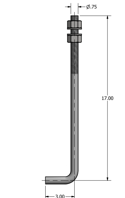
Ø.75 X 20.00 ANCHOR BOLT
